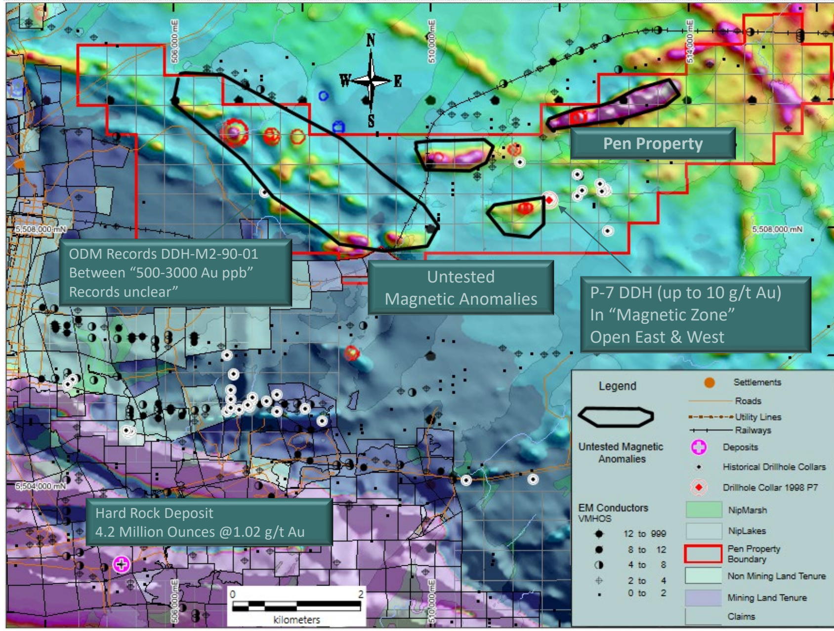
GERALDTON-TASHOTA AREA, Ontario Airborne Magnetic and Electromagnetic Surveys. Geophysical Data Set 1031
